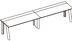
Single Bench w/Straight Mid-leg and Cable Cover for 2 People 单边共享台带直形中脚及走线盖: 2人 W: 2400^, 2800, 3000, 3200, 3600 D: 800, 900, 950 H: 725
