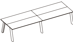
Double Bench w/A-Shape Mid-leg for 4 People 双边共享台带A形中脚: 4人 W: 2400^, 2800, 3000, 3200, 3600 D: 1200, 1400, 1500 H: 725
