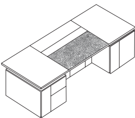
Executive Desk, w/o Extension/Return Cabinet W3200 D1150 H760 W3000 D1150 H760 W2800 D1150 H760
