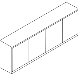
Low Cabinet, w/Wooden Doors W2400 D470 H760
