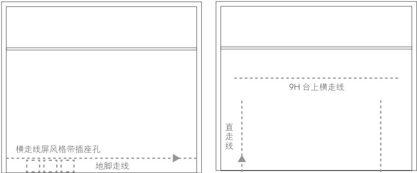
Cabling and Socket Cut Outs at Floor Level
